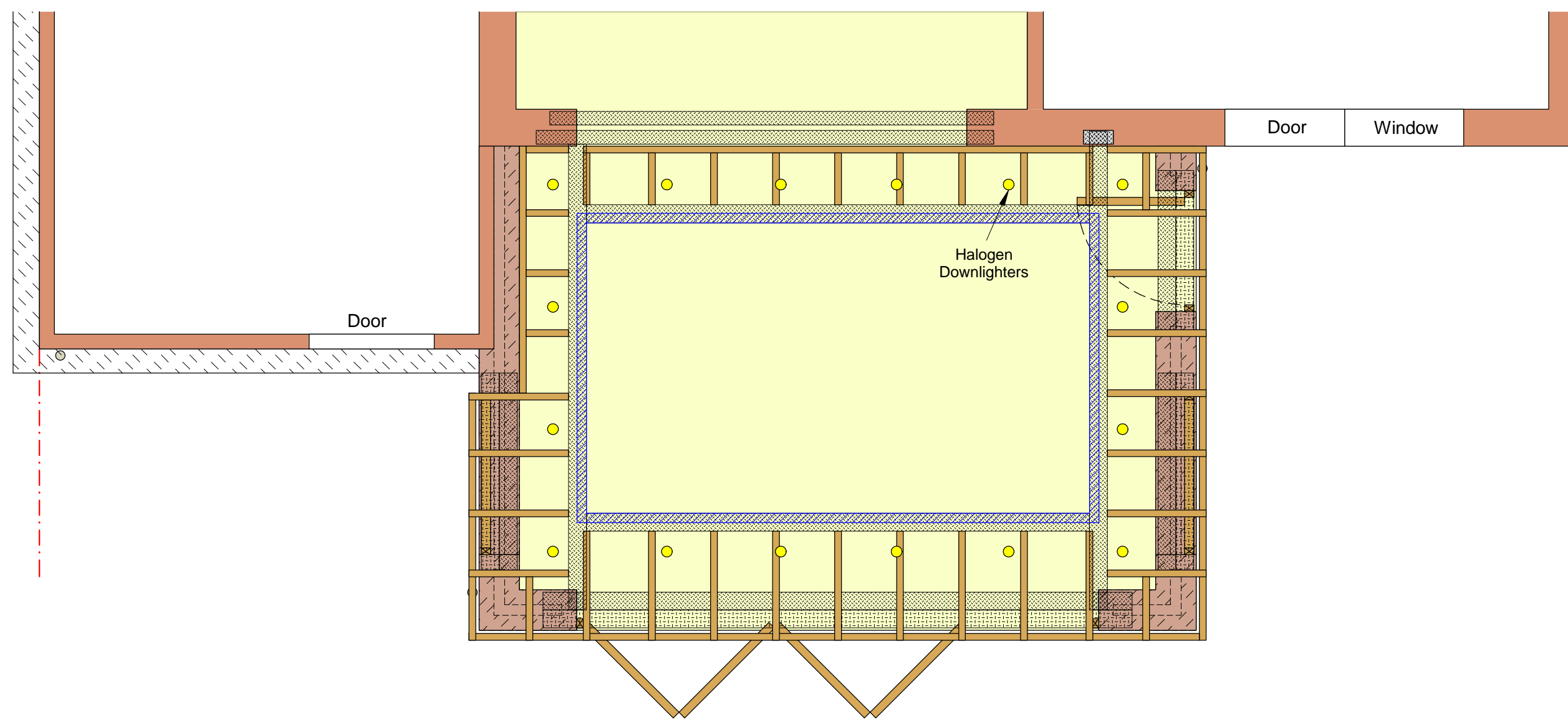
ROOF LAYOUT
