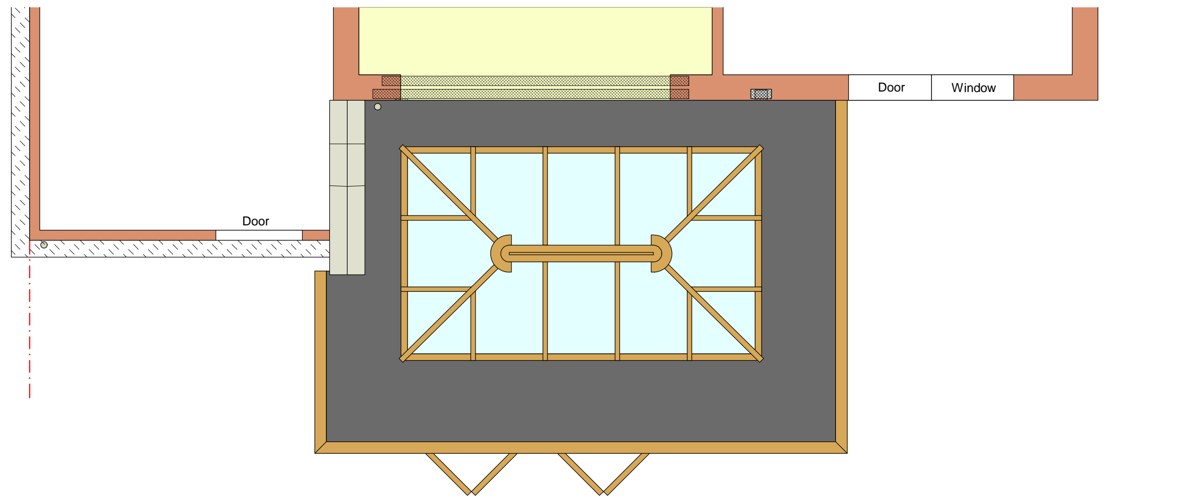
PLAN VIEW
