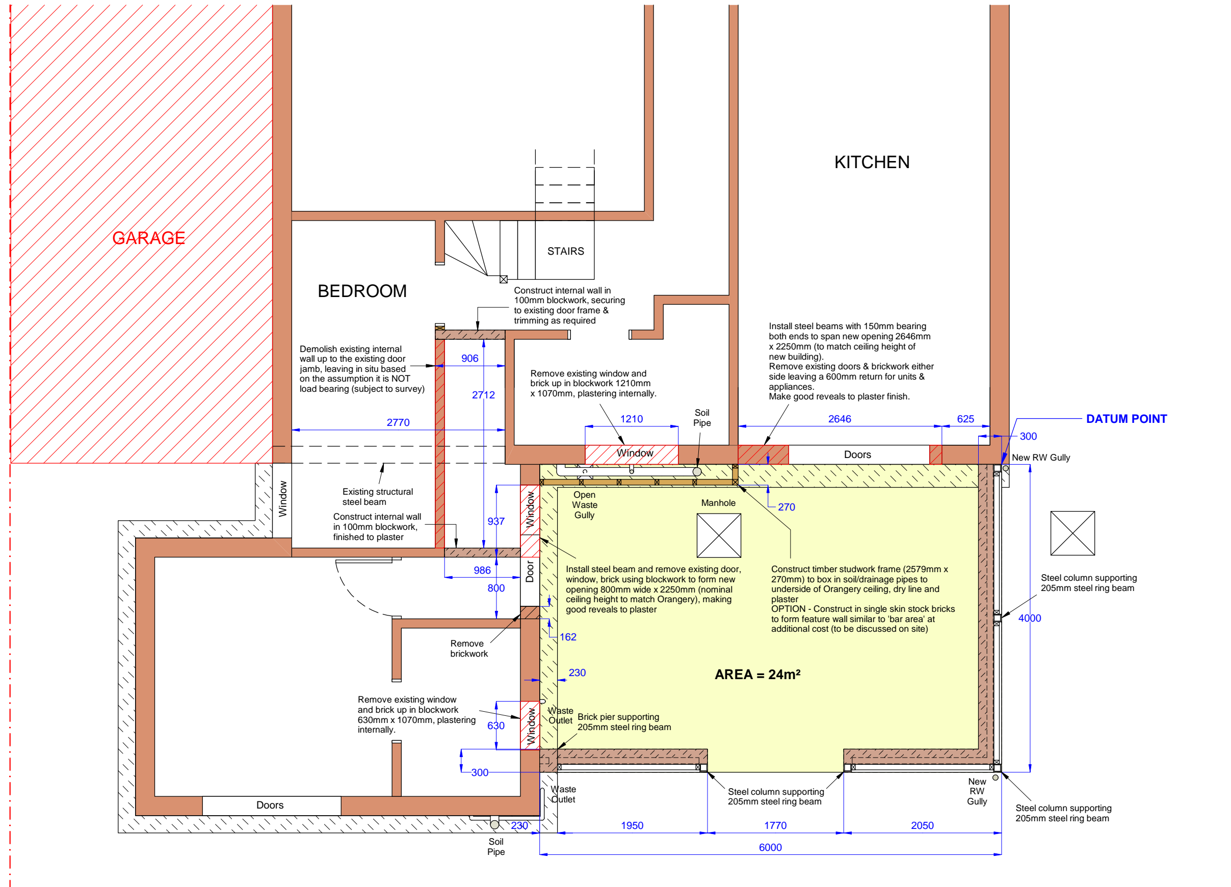
BASE PLAN
